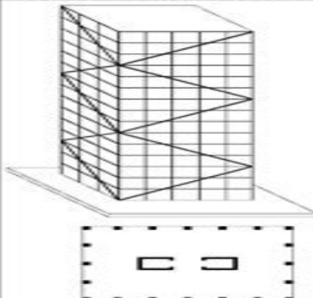
Braced-Tube System
