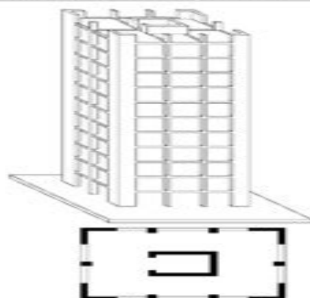
Frame-Tube System
