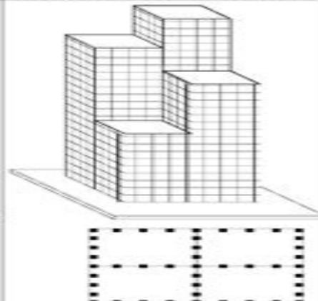
Bundled-Tube System
