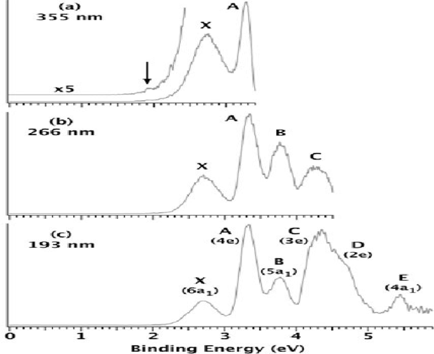
Fig. 1. Photoelectron spectra of Al-NT at (a) 355 nm (3.49 eV), (b) 266 nm (4.66 eV), and (c) 193 nm (6.42 eV).
