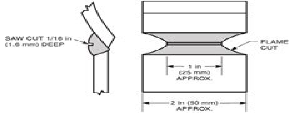
(B) POINT SPECIMEN
