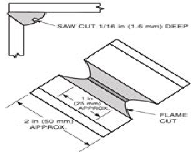
(C) CROTCH SPECIMEN
