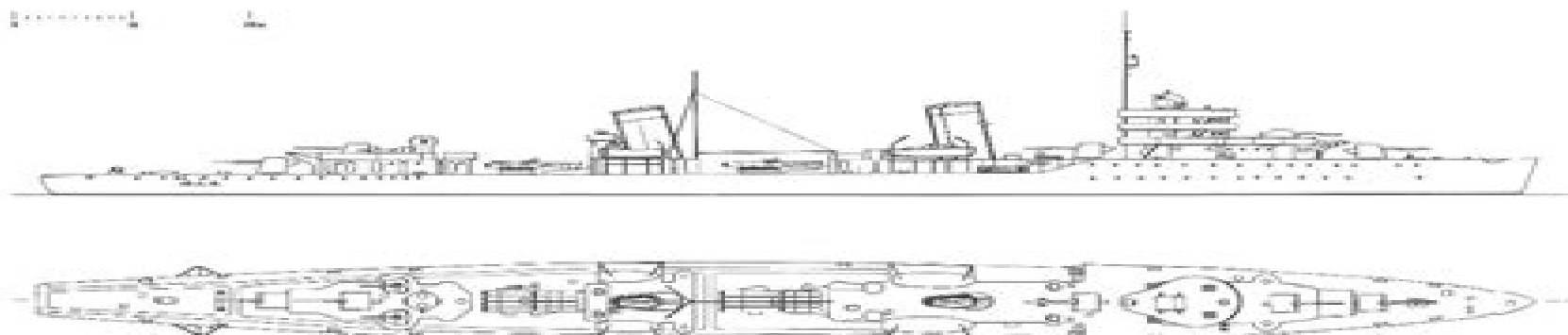
Leningrad class destroyer Baka, as originally planned. (Drawing: S Breyer, 1935)
