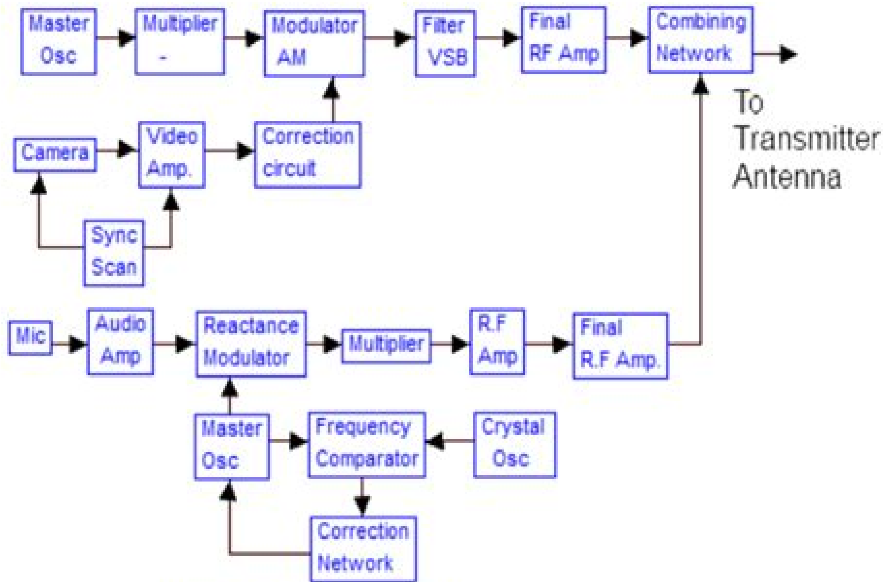
Fig (b) Complete T.V transmitter
