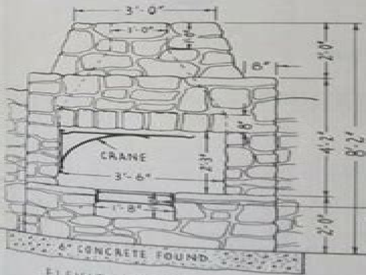
ELEVATION VIEW
