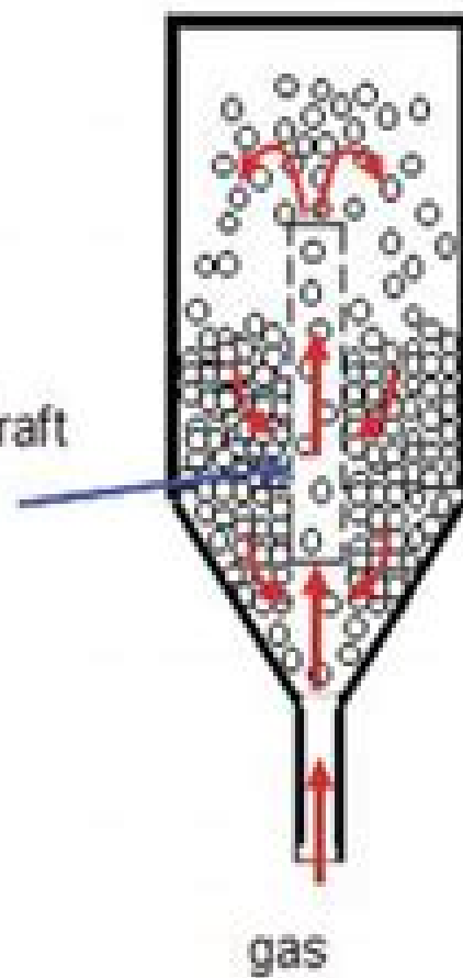
Spouted bed apparatus with porous draft tube
