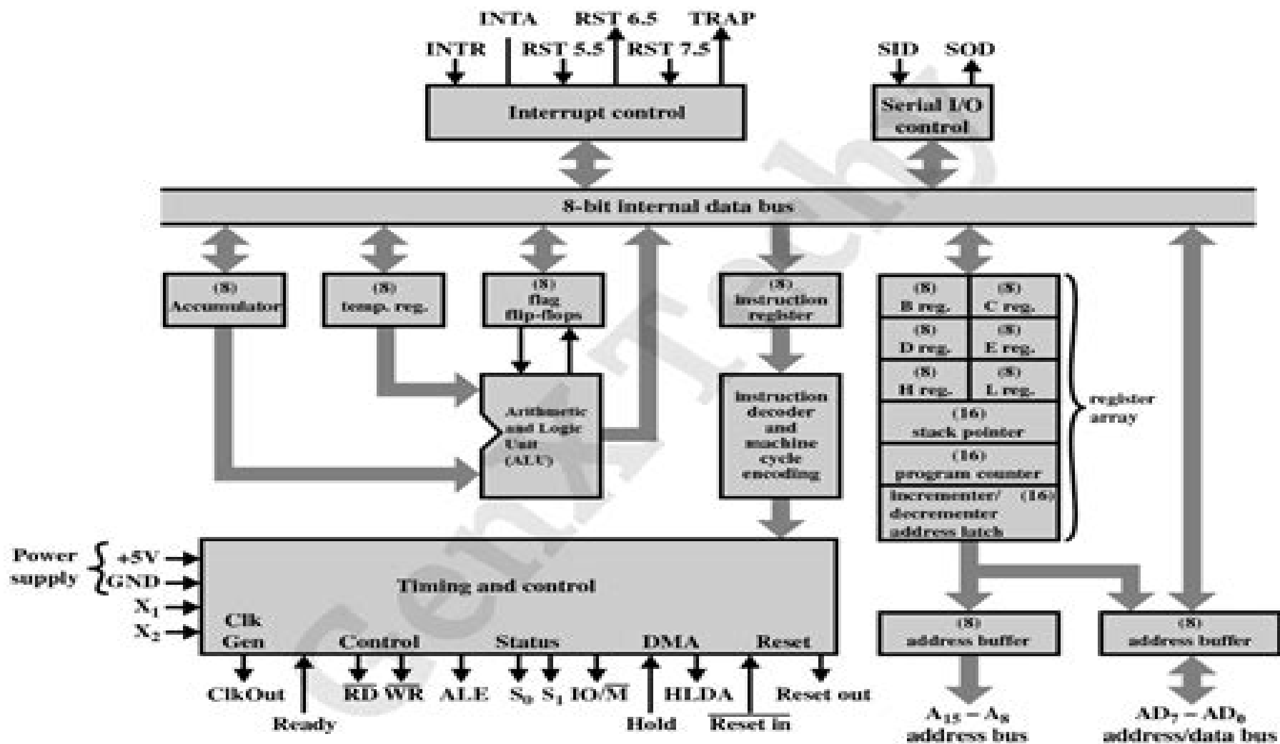
Fig. 1: Block diagram of 8085 microprocessor
