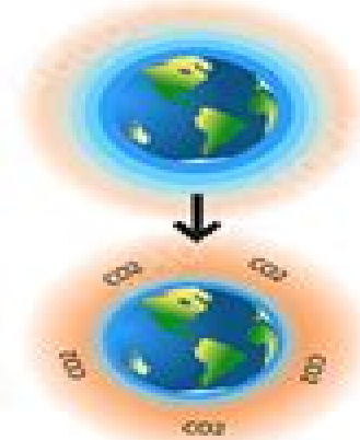
Greenhouse Effect
