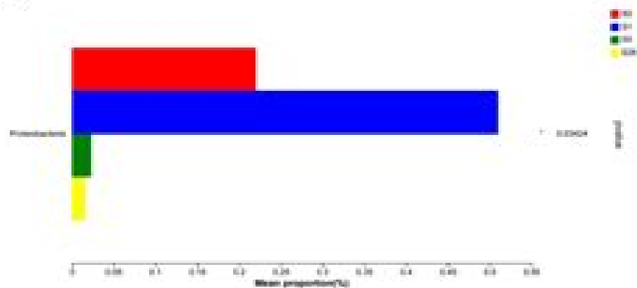
One-way ANOVA bar plot
