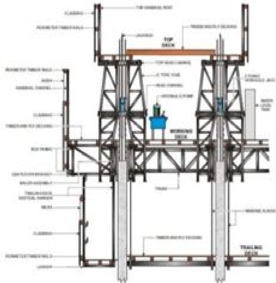
TYPICAL SECTION THROUGH SLIPFORM SYSTEM FOR VERTICAL STRUCTURES
