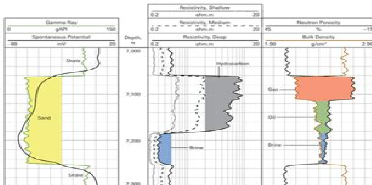
Figure 1. A basic log. A suite of logging measurements might include spontaneous potential, gamma ray, resistivity, neutron and density curves in a single presentation. The gamma ray response (Track 1) distinguishes the low gamma ray value of sand from the higher value of shale. The spontaneous potential curve generally follows a trend similar to that of the gamma ray. The next column, called the depth track, indicates the depth at which the measurement was made. Across the sandstone formation, the resistivity measurements (Track 2) are noticeably higher in the hydrocarbon zone than in the water-saturated zone in the lower part of the sand. Both neutron porosity and bulk density (Track 3) provide measures of porosity. Within the hydrocarbon-bearing zone, the separation of the curves varies depending on the type of fluid encountered.
