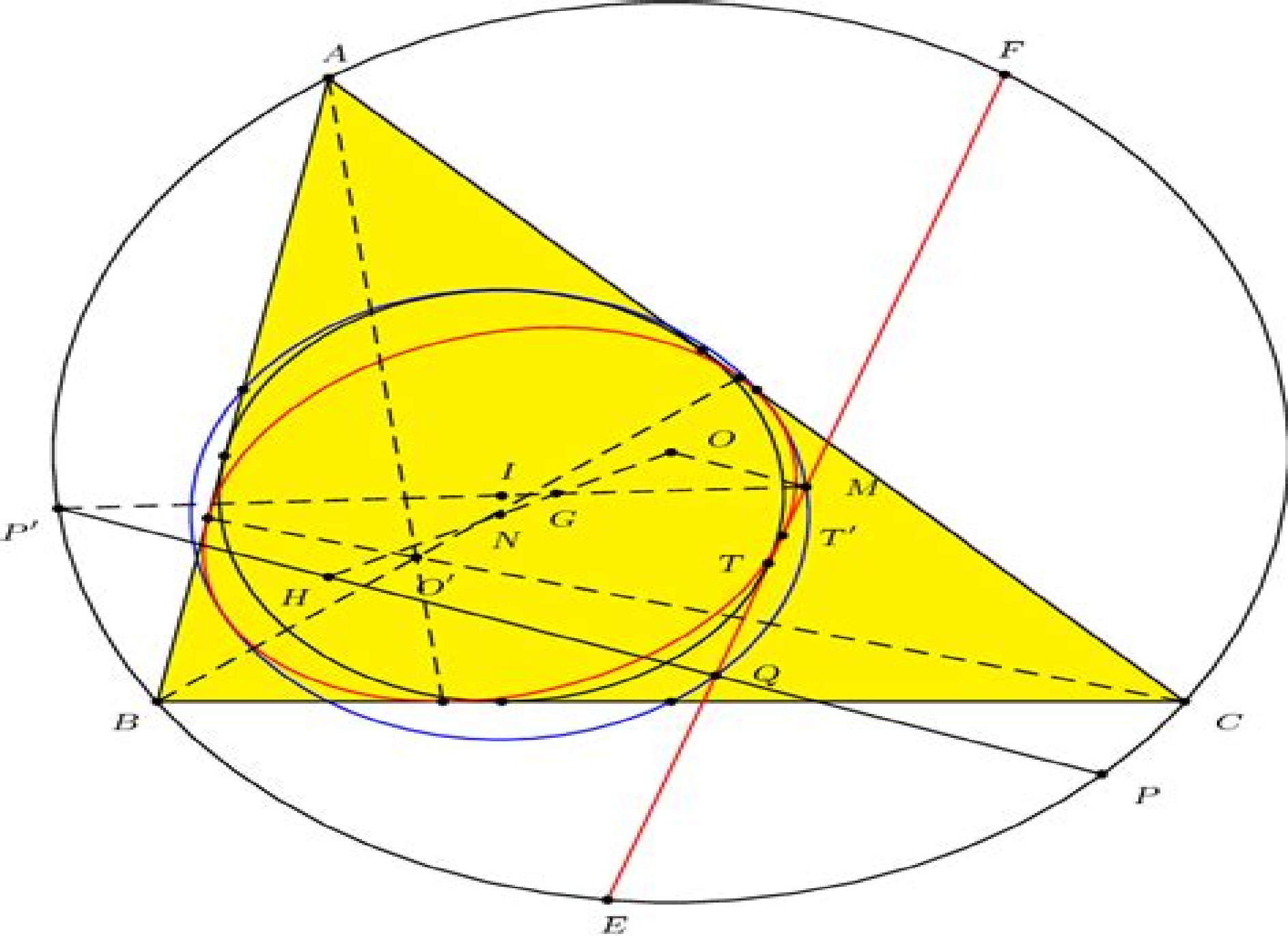
Figure 2. The fourth side of a triangle as a common tangent
