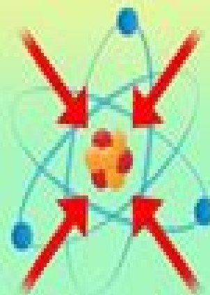
STRONG FORCE
