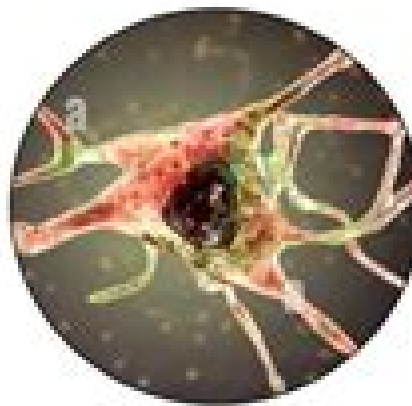
Healthy neurons
