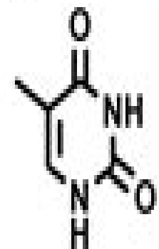
Thymine
