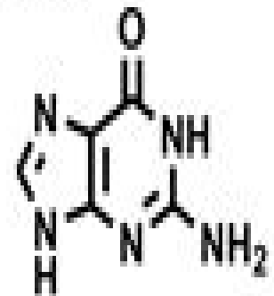
Guanine
