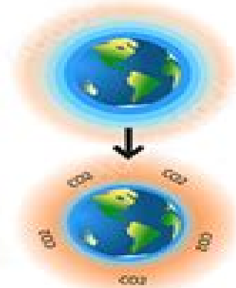
Greenhouse Effect
