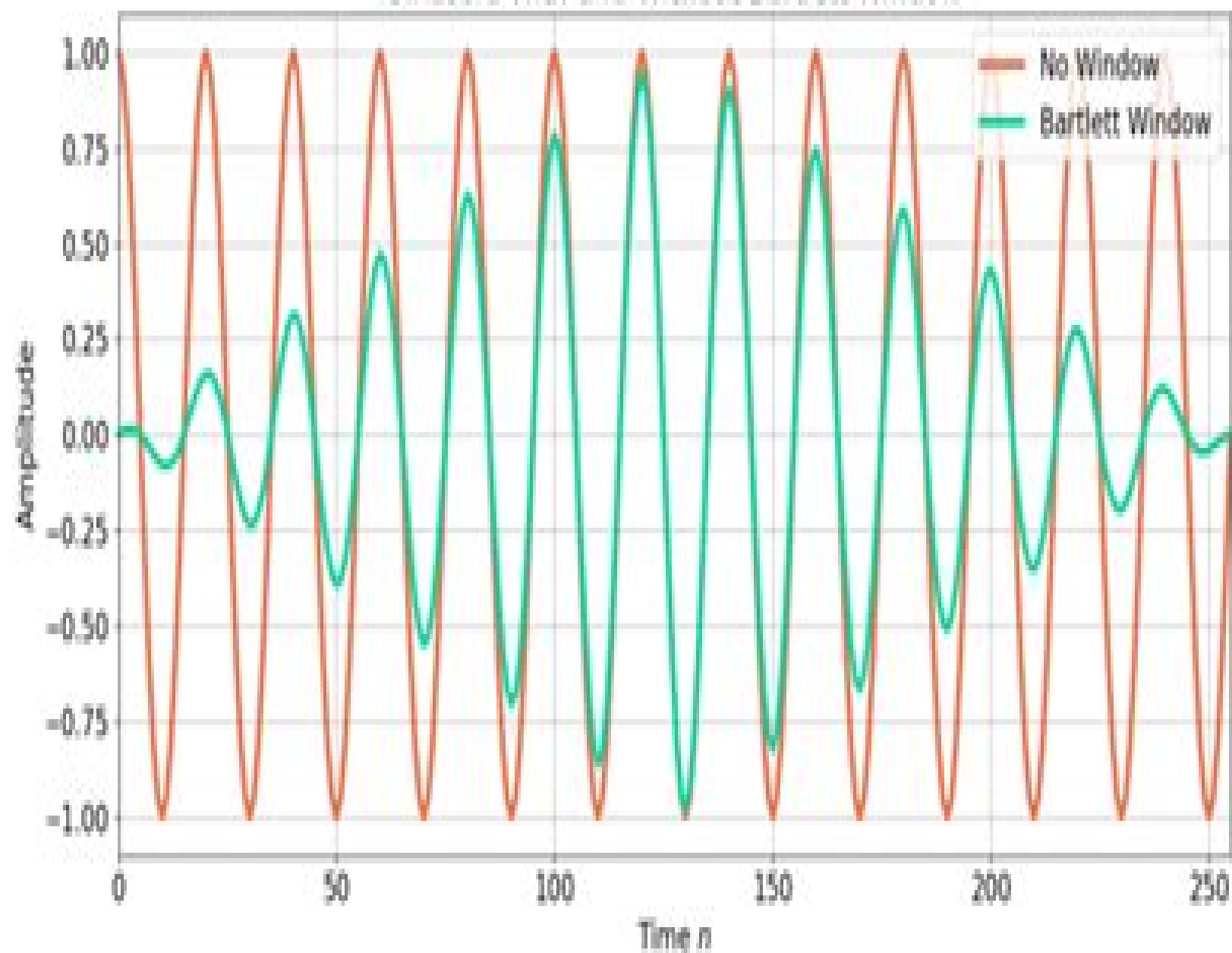
Sinusoid With and Without Bartlett Window
