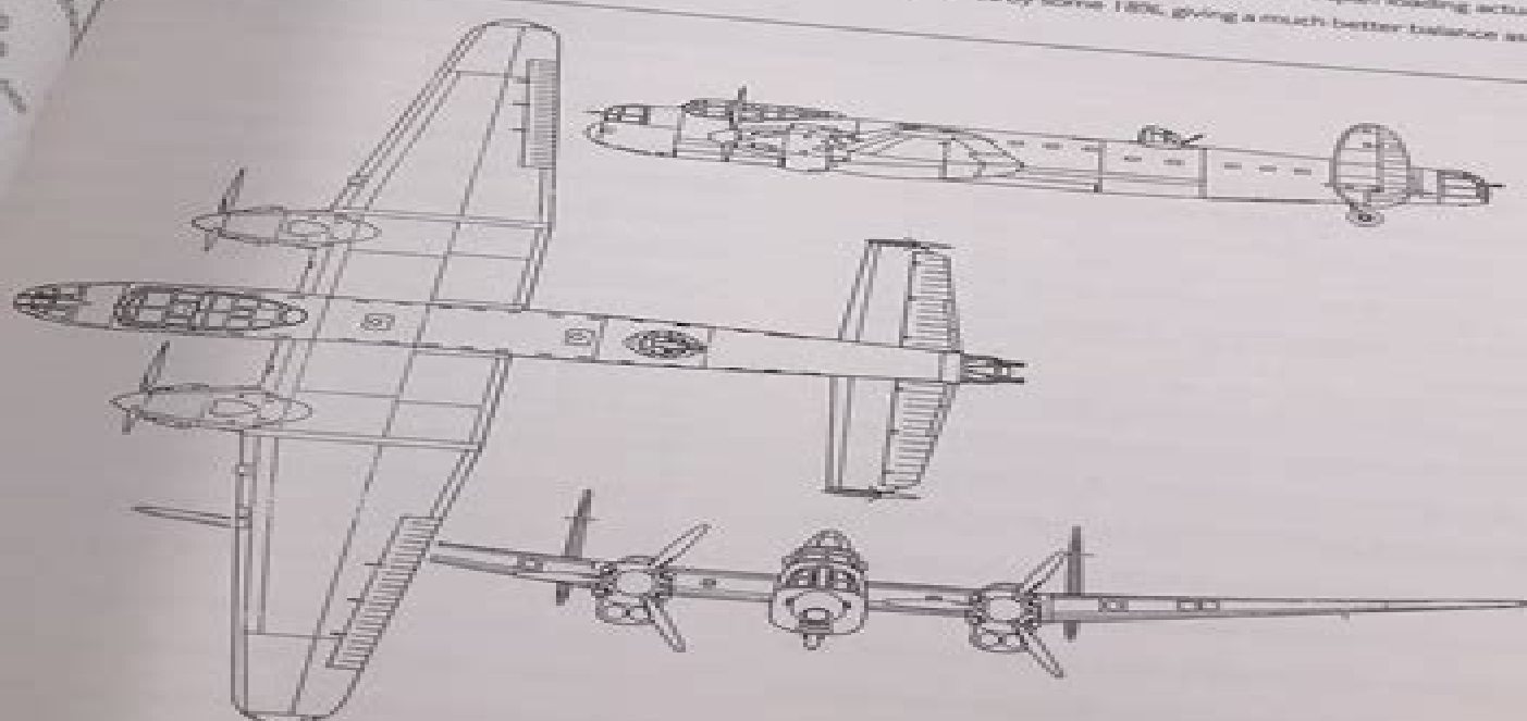
Avro Type 679 Manchester. Final production configuration, with 90ft wing span, 33ft tailplane span and 12ft high fins, fitted with Frazer-Nash FN7 dorsal gun turret.
