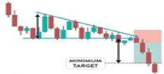
Descending Triangle
