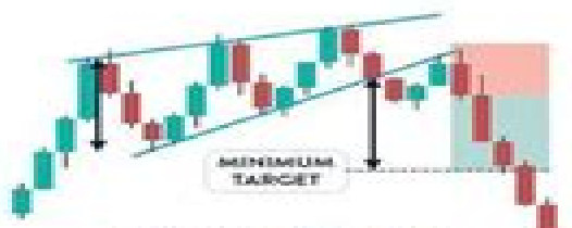
Rising Wedge
