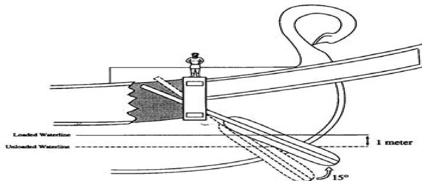
Figure 2.1 The effect the height of the rudder mount above the water has on the shaft angle of a quarter-rudder floating at equilibrium.
