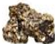
pyrite
