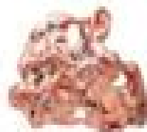
native copper
