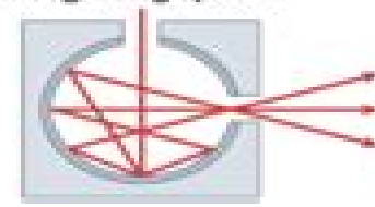
Integrating sphere
