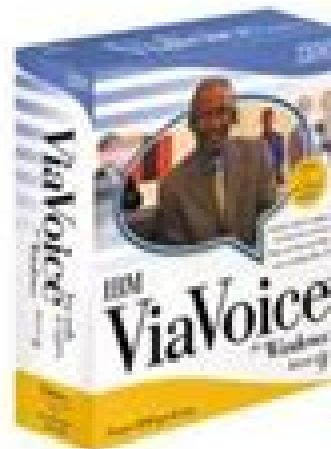
IBM ViaVoice
