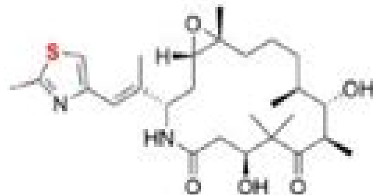
Ixabepilone (anticancer drug)
