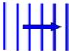
Plane wave
