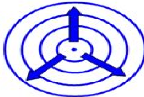
Circular wave
