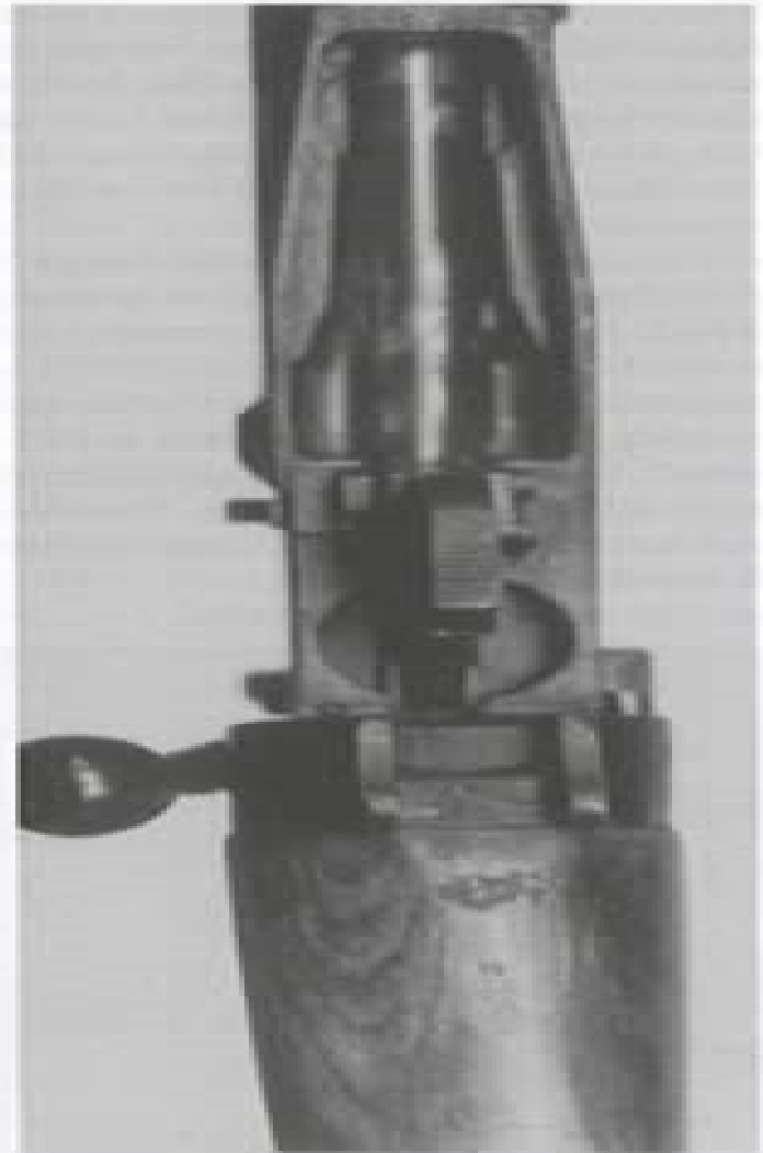
These two views of the Number 5 rifle show some of the lightening cuts which were made in order to shave weight from the rifle. At left, the dished out cuts in the barrel's chamber area are quite evident, while at right, metal at the bottom of the receiver was judiciously removed.
