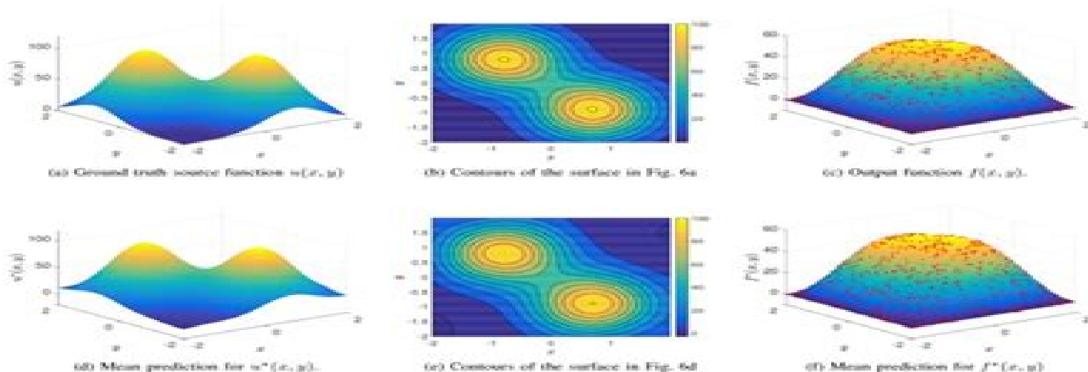
Fig. 6. The upper row shows the ground truth data for the 2D PDE Poisson example: the input source (Fig. 6a); contours of the ground truth input source (Fig. 6b); ground truth for the output function (Fig. 6c). Noisy observations are shown as red crosses in Fig. 6c. The lower row shows the predicted mean function \mathbb{E}[u^*(x, y)|\mathcal{Y}] (Fig. 6d); contours of the predicted mean function (Fig. 6e); the predicted mean output \mathbb{E}[f^*(x, y)|\mathcal{Y}] (Fig. 6f). Noisy observations are again shown as red crosses in Fig. 6f.
