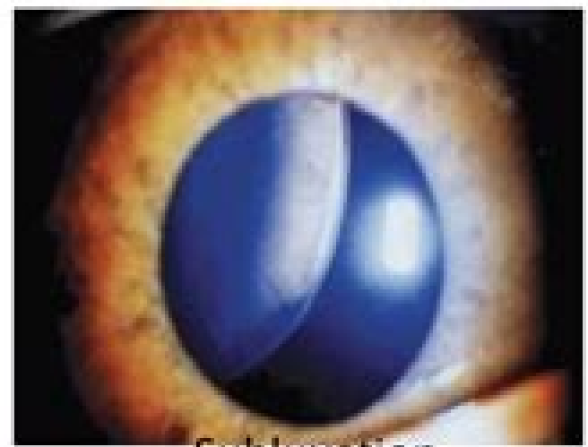
Subluxation
