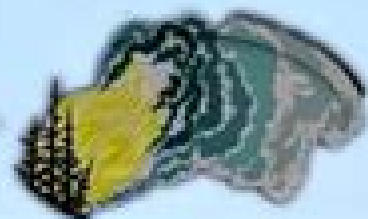
Forest fires
