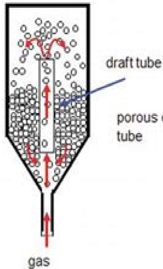
Spouted bed apparatus with draft tube
