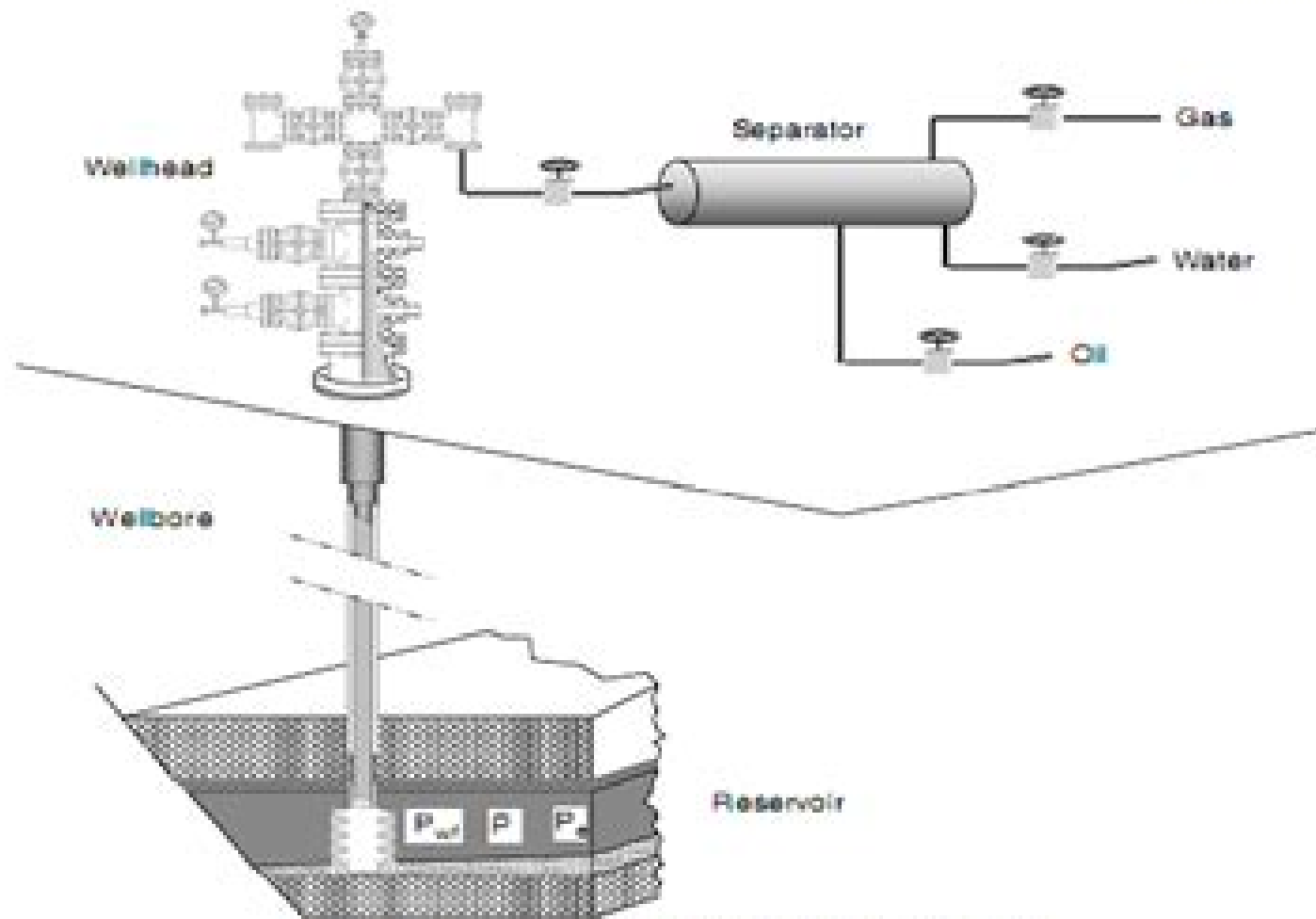
Figure 1.1 A sketch of a petroleum production system.
