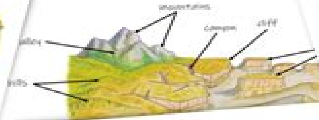
sand dune
