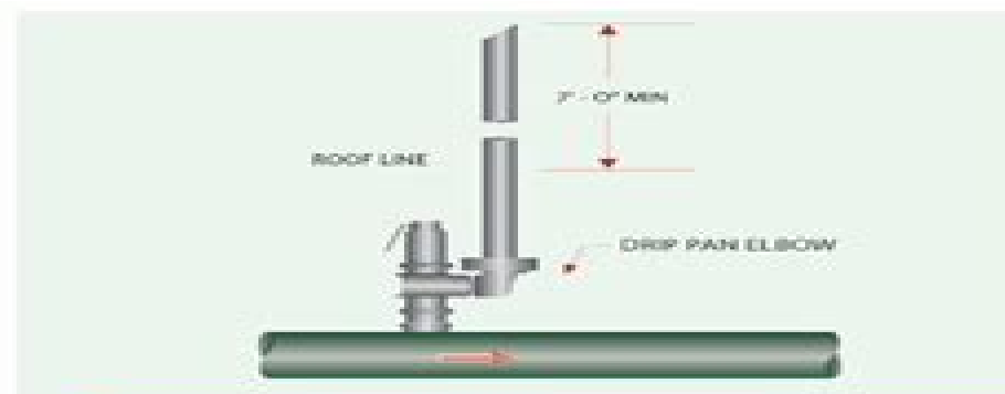
Figure 2: Steam Safety Valve on a Steam line
