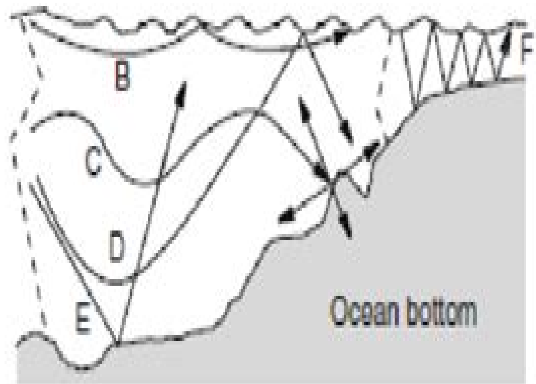
Ocean basin
