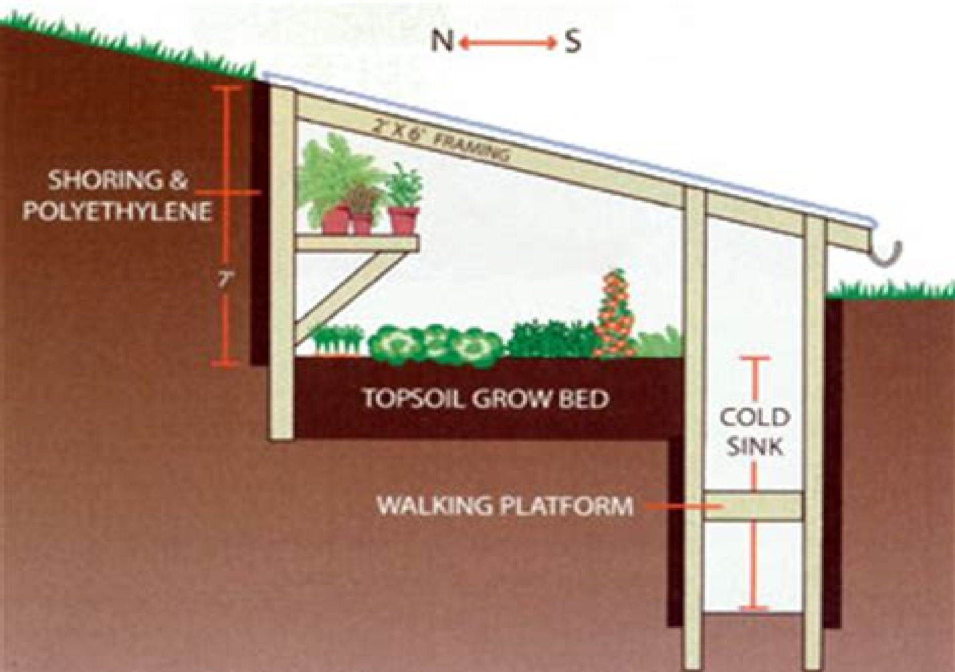
Cross Section of Earth-sheltered Greenhouse
